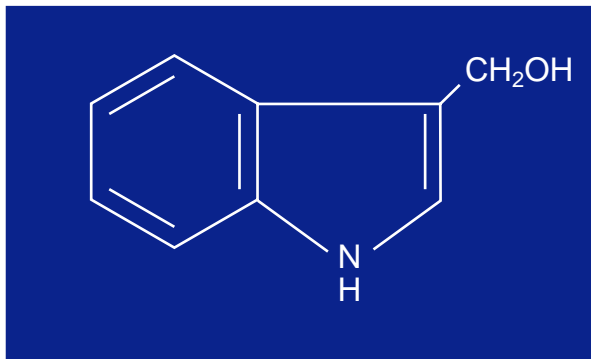
Figure 1: Indole-3-Carbinol.
